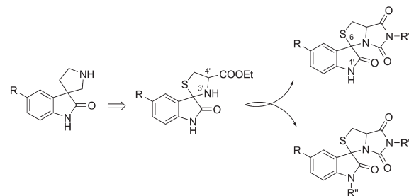
Figure 2. Design of new derivatives from spiro(oxindole-3,3'-thiazolidine): R = H, CH_3, Br ; R' = benzyl derivatives or alkyl; R'' = H or acyl derivatives.
