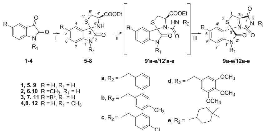
Scheme 1. Synthesis of Spiro[imidazo[1,5- c ]thiazole-3,3'-indoline]-2',5,7(6 H ,7 aH )-trione Derivatives 9a–e / 12a–e a
