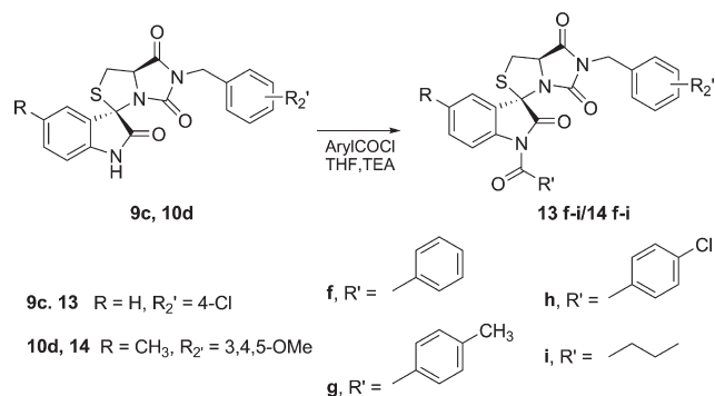
Scheme 2. Synthesis of 1'-Acylspiro[imidazo[1,5-c]thiazole-3,3'-indoline]-2',5,7(6 H ,7 aH )-trione derivatives ( 13f–i / 14f–i )
