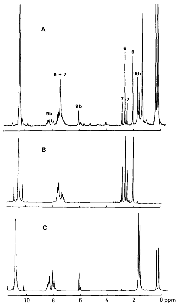
Fig. 1. ^1\text{H} -NMR. spectra (60 MHz) in \text{HSO}_3\text{F}/\text{SO}_2\text{ClF} at 0^\circ to 10^\circ . – A. Product mixture formed from 1a . The signals at \delta \approx 0 –0.5 are due to decomposition of TMS, those at \delta > 10 to \text{HSO}_3\text{F} . – B. Mixture of 6 and 7 , formed from 2a . – C. 9b formed from 8 .
