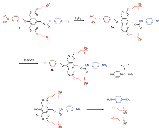
Scheme 1. Disassembly Pathway of AB 3 Self-Immolative Dendron 3 , Initiated by a Trigger That Is Cleaved by Hydrogen Peroxide (Blue, 4-Nitroaniline Reporter; Red, Choline Units That Trigger Further Dendron Disassembly)
