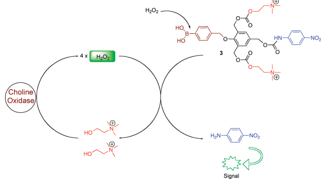
Figure 3. DCR system based on a hydrogen peroxide trigger and choline.
