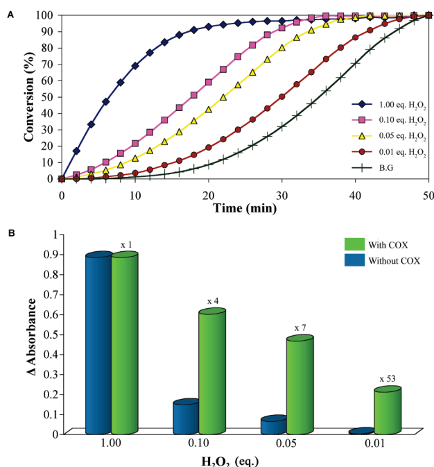
Figure 4. (A) Release of 4-nitroaniline from dendron 3 (500 \mu M) in the presence of COX (0.3 mg/mL) in PBS (pH 7.4) upon addition of buffer only (B.G.) or the indicated amounts of H 2 O 2 monitored at 405 nm over time. (B) Comparison of signals measured in the presence of COX by the DCR amplification technique (green) vs signals measured using dendron 3 as a classic probe (i.e., without COX) (blue). The background signal present at 25 min was subtracted from the values shown.
