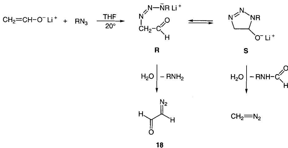
Scheme 7
