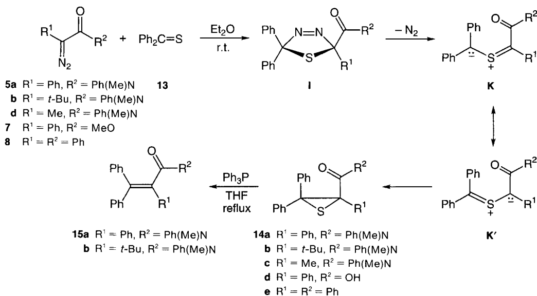
Scheme 5
