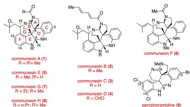
Figure 1. Communesins (1–8) and perophoramidine (9).
