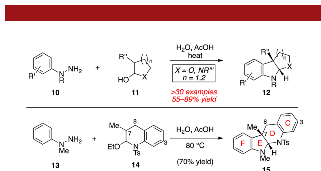
Figure 2. Interrupted Fischer indolization methodology and approach toward alkaloids 1–9.
