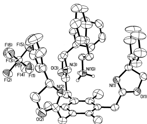
Figure 1. The X-ray crystal structure of 4 ·PhCH 2 CH 2 NH 3 + PF 6 − (except for the NH 3 + hydrogen atoms, hydrogen atoms have been omitted for clarity). Selected interatomic distances [Å] and angles [°]: N(1G)···N(1) 2.972, N(1G)···N(2) 3.016, N(1G)···N(3) 2.983; N(1)–N(1G)–N(2) 124.1, N(1)–N(1G)–N(3) 109.9, N(2)–N(1G)–N(3) 109.6.
