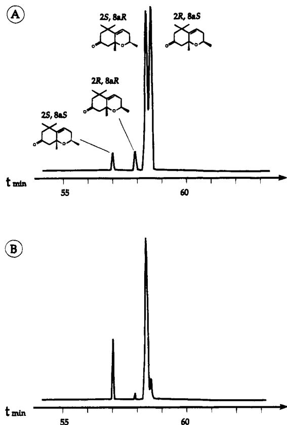
Figure 2. MDGC [DB-Wax/octakis(2,6-di- O -methyl-3- O -pentyl)- \gamma -cyclodextrin] enantiodifferentiation of 3,4-dihydro-3-oxoedulan isomers 1a–d: (A) separation of the racemic synthetic mixture and appointed absolute configuration; (B) enantiodifferentiation in a natural sample (passion fruit, Africa).
