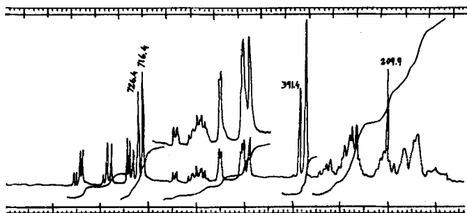
Figure 3—NMR spectrum of mixture rich in I.
