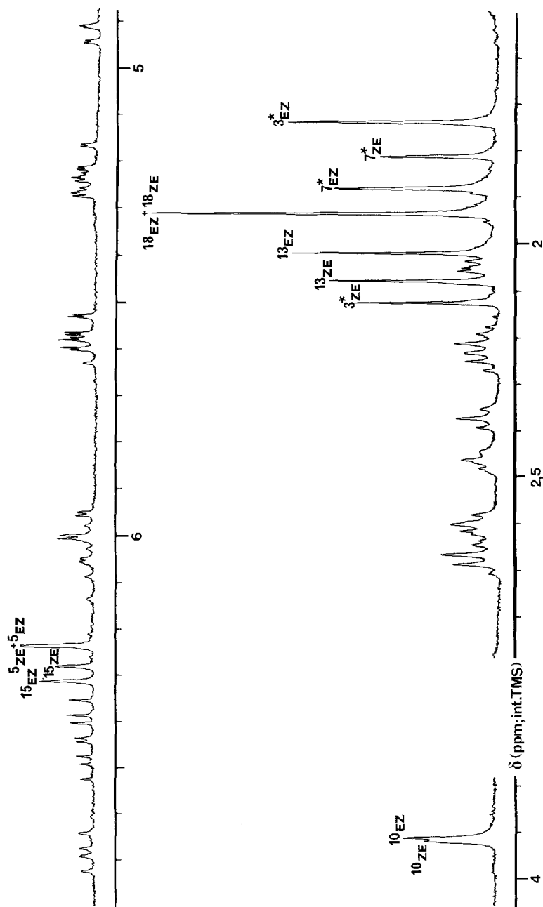
Fig. 4. ^1\text{H} -NMR spectrum of (Z,E) -1 + (E,Z) -1 in \text{CD}_3\text{OD} (360 MHz). Assignments marked with an asterisk are uncertain and may be interchanged within the corresponding diastereomer. The signals of the four propionic acid side chains (2.0–2.75 ppm) and the four vinyl groups (4.9–6.8 ppm) could not be assigned with confidence due to overlap
