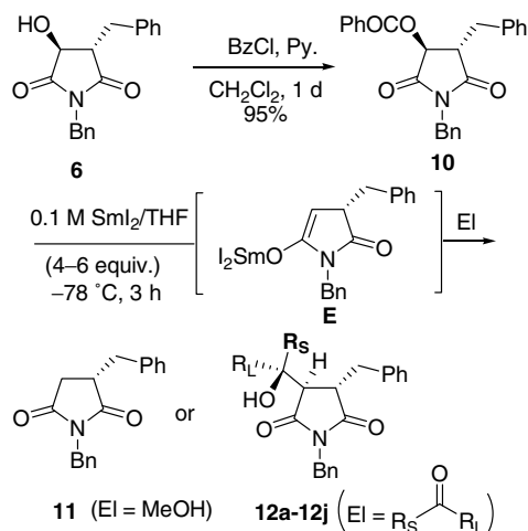
Scheme 3. \text{SmI}_2 -promoted deoxygenation-coupling reactions of 10 .
