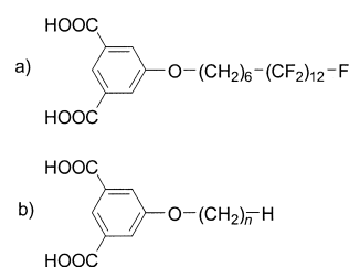
Figure 1. Chemical structure of the compounds under investigation: (a) 5-(( \omega -perfluorododecyl)hexyloxy)isophthalic acid (F 12 H 6 -ISA); (b) 5-( \omega -alkoxy)isophthalic acid (H n -ISA, n = 18, 20 ).
