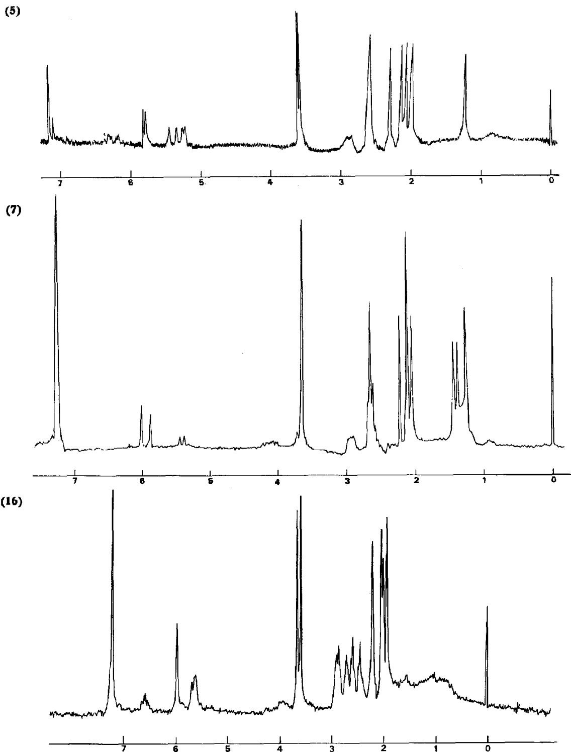
Fig. 3. Spectres RMN. (dans \text{CDCl}_3 ) des esters méthyliques de: phorcabiline (5) (90 MHz), isophorcabiline (7) (90 MHz), néobiliverdine \delta (16) (240 MHz) (7,27 ppm = \text{CHCl}_3 ; 1,27 ppm = impureté).
