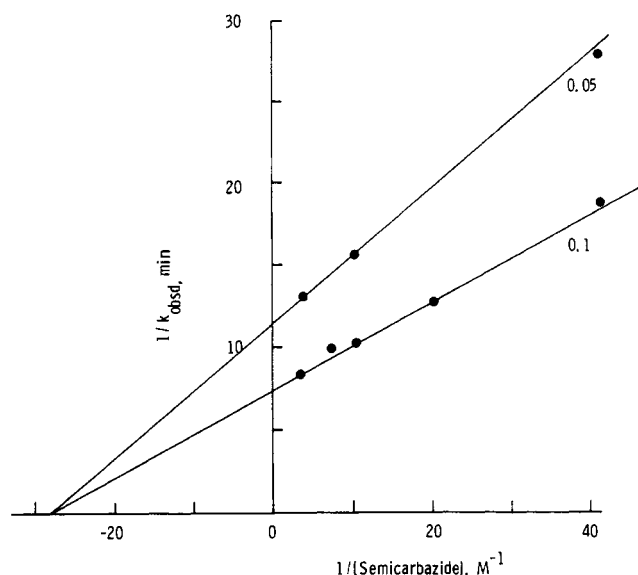
Figure 5. Double reciprocal plot of k_{\text{obsd}} vs. [semicarbazide] for semicarbazone formation from N -propylpyruvamide at pH 5 and two phosphate buffer concentrations (0.05 and 0.1 M). Ordinal intercepts are reciprocal of k_2^{\text{H}}[\text{H}] + k_2^{\text{PO}_4}[\text{PO}_4] ; abscissal root is K_1/(1 + K_{\text{hyd}}) .
