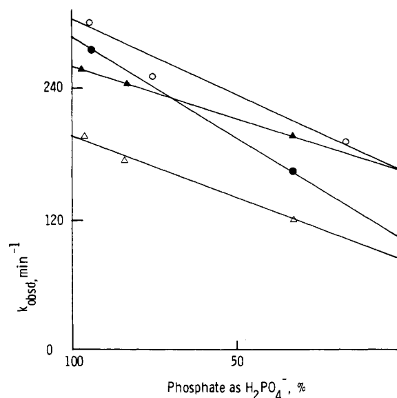
Figure 4. Dependence of k_{\text{obsd}} for reaction of semicarbazide with four pyruvamides at constant semicarbazide (0.05 M) and total phosphate (0.1 M) concentration upon fraction of phosphate present as \text{H}_2\text{PO}_4^- (as opposed to \text{HPO}_4^{2-} ). (O) pyruvamide; (●) N -propylpyruvamide; (Δ) pyruvoylphenylglycine; (▲) pyruvanilide.
