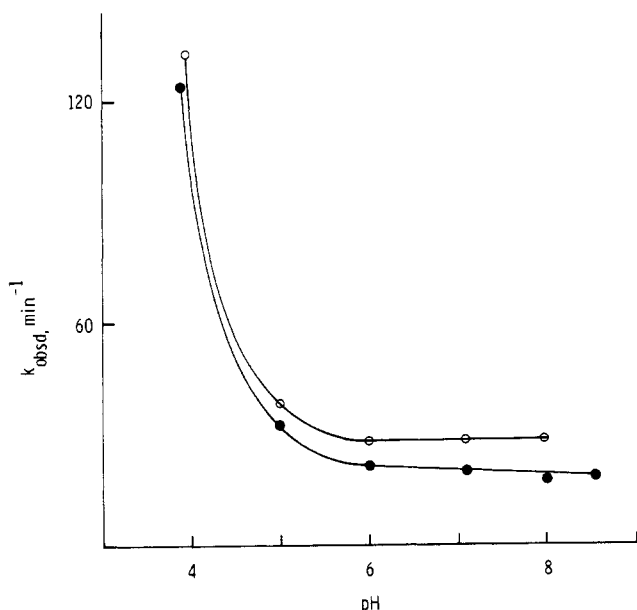
Figure 1. Dependence of rate of carbinolamine formation from semicarbazide and pyruvamide (O) or N -propylpyruvamide (●) upon pH. Values of k_{\text{obsd}} at 0.05 M semicarbazide, are extrapolated to zero buffer (phosphate) concentration, and at pH 3.9 are corrected for protonation of semicarbazide.
