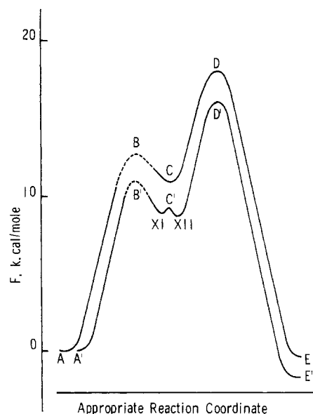
Figure 6. Estimated energy profiles for water catalyzed reaction of N,N -dimethylpyruvamide (A) and pyruvamide (A') with semicarbazide. E,E' are product carbinolamines; C,C' are metastable carbinolamine zwitterion and/or carbinolamine-isoamide intermediates.
