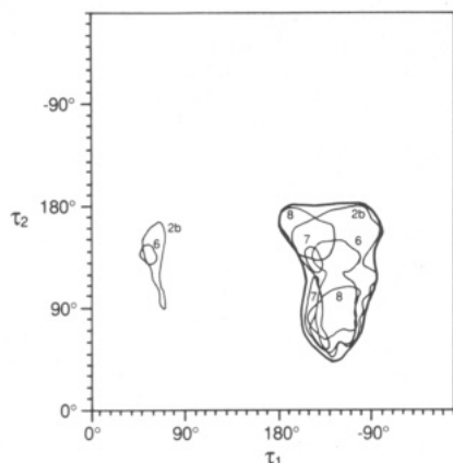
Figure 7. Union of the 3 kcal/mol contours for 2b and the methyl-truncated analogues of 6 , 7 , and 8 , enclosed by the heavy line.
