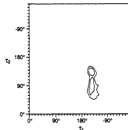
Figure 5. Conformational map for the methyl-truncated analogue of 7 . Energy contours are at 3 and 6 kcal/mol above the global minimum.
