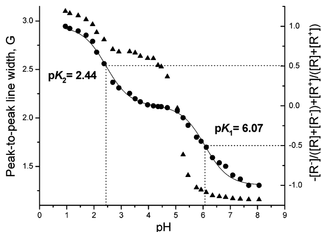
FIGURE 5. Experimental pH dependence of the line width of the EPR spectrum central nitrogen hyperfine component of the nitroxide 13b in 1 mM Na-phosphate buffer solution in the presence of 32 mM K_3[Fe(CN)_6] (▲) and corresponding calculated values of the term (-[R^-]/([R] + [R^-]) + [R^+]/([R] + [R^+])) (●), where R^- and R^+ represent deprotonated and protonated forms of the nitroxide, respectively, and R represents uncharged zwitterion form. At pH below 4.0, the above term is equal to the fraction f of the radical in protonated form ( f(R^+) = [R^+]/([R] + [R^+]) and [R^-] \approx 0 ). At pH above 4.0, the term is equal to the fraction of the radical in deprotonated form ( f(R^-) = [R^-]/([R] + [R^-]) and [R^+] \approx 0 ) taken with sign minus, -f(R^-) , to keep similar graphic representation for the experimental (▲) and calculated (●) dependencies. The solid line represents the nonlinear least-squares fit of the data to the Henderson–Hasselbalch equation, yielding pK_1 = 6.07 and pK_2 = 2.44 .
