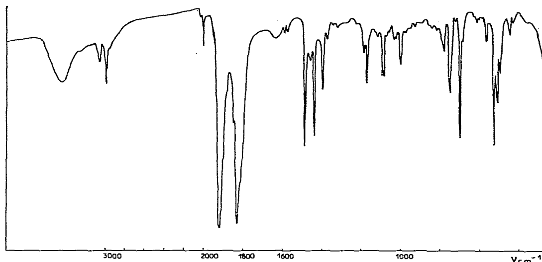
Fig. 3. Infrared spectra of solid complex (\text{C}_2\text{H}_5)_4\text{N}[(\eta\text{-C}_3\text{H}_5)(\text{CO})_2\text{WCl}_2\text{PPh}_3] .
