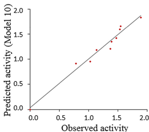
Fig. 10. Observed versus predicted activity for model 10.
