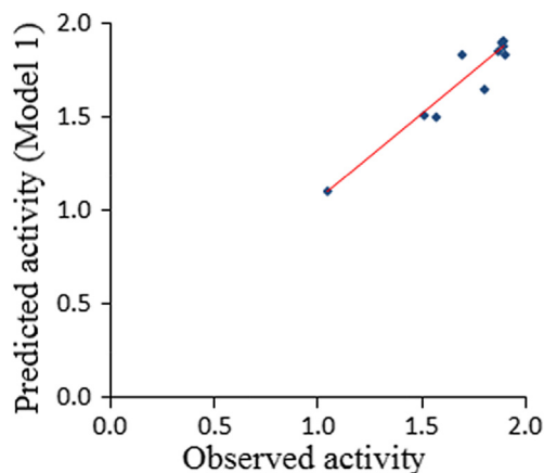
Fig. 1. Observed versus predicted activity for model 1.
