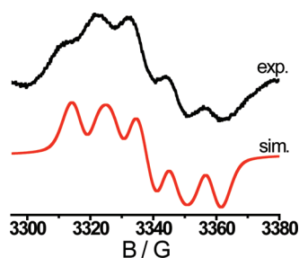
Figure 7. X-band EPR spectrum of electrochemically generated 4^{+\bullet} in \text{CH}_2\text{Cl}_2/0.1 \text{ M Bu}_4\text{NPF}_6 at 233 K (black = experimental, red = simulated).
