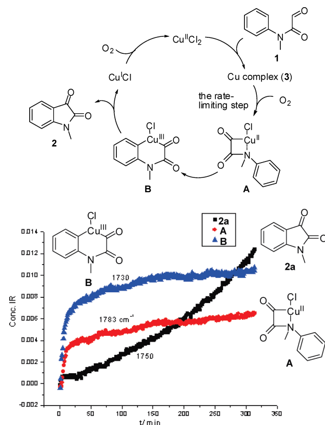
Figure 1. Data of in situ FTIR analysis during the reaction of Cu complex under air atmosphere.
