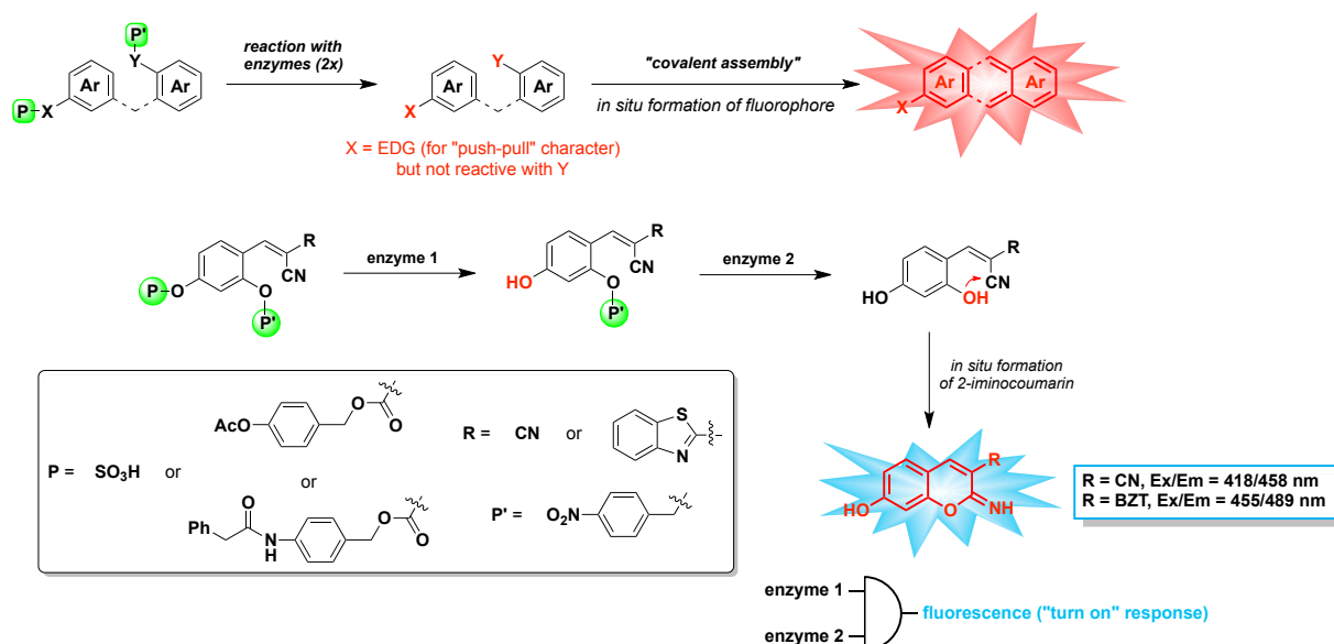
Fig. 1 Strategy explored in this work: (top) "covalent assembly" principle applied to the simultaneous detection of two distinct enzymes (X = NH or O, EDG = electron-donating group); (bottom) in situ synthesis of 3-substituted-7-hydroxy-2-iminocoumarin scaffolds from a non-fluorescent caged precursor and through domino reactions triggered by the two different enzymes (failed attempt: probe for sulfatase-NTR, R = CN, P = SO 3 H and P' = para -nitrobenzyl; probes for PLE-NTR, R = BZT or CN, P = Ac-PHBoxycarbonyl and P' = para -nitrobenzyl; probe for PGA-NTR, R = CN, P = PhAc-PABoxycarbonyl and P' = para -nitrobenzyl). BZT = 2-benzothiazolyl, NTR = nitroreductase, PLE = pig liver esterase and PGA = penicillin G acylase.
