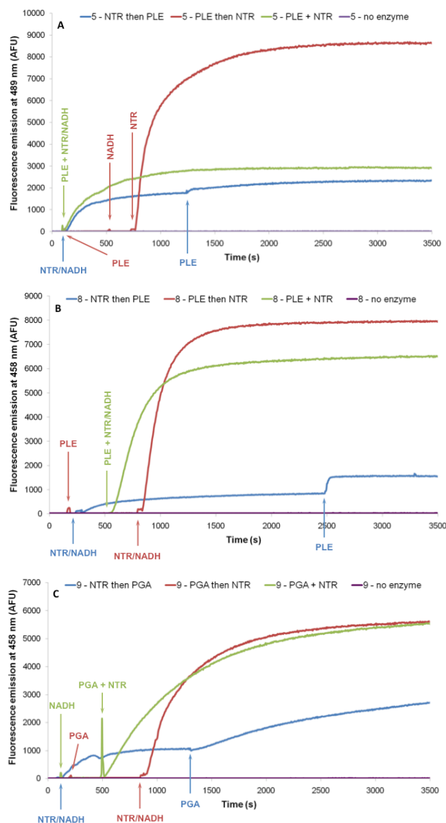
Fig. 2 Time-dependant changes in the blue/green fluorescence intensity of fluorogenic "turn-on" probes 5 , 8 and 9 (concentration: 1.0 \mu M) in the presence of two distinct enzymes in PB at 37 ^{\circ} C (see ESI † for more details about sequential and simultaneous incubations protocols with NTR (0.1 U) / NADH (45 \mu M), PLE (1 U) and PGA (1 U)). (A) Ex./Em. 455/489 nm; (B)-(C) Ex./Em. 418/458 nm. For each probe, a further kinetic curve (purple trace) was recorded under the same conditions but without enzymes and co-factor.
