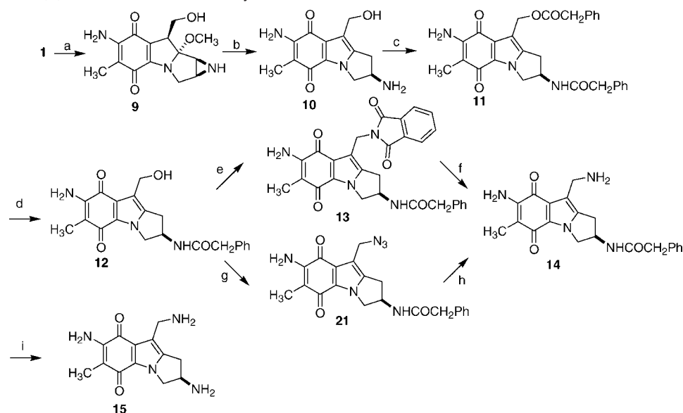
Scheme 2. Synthesis of 2,7,10-Triamino-10-decarbamoylemitosene 15 a
