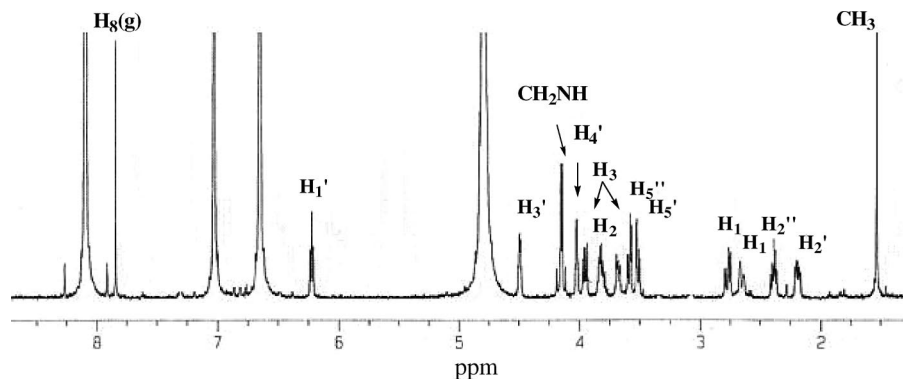
Figure 2. ^1\text{H} NMR spectrum of 8 in pyridine- d_5 /D _2 O. H 8 (g), 8-proton of guanine.
