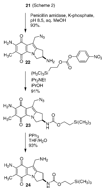
Scheme 5. Synthesis of N 2 -Protected 2,7,10-Triaminomitosenes ( 24 )
