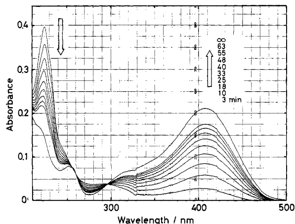
Figure 1. Visible spectral change of the photobleached 2 ( 1.0 \times 10^{-5} M) as a function of time for the thermocoloration in the dark in an aqueous buffered solution (pH 5) at 25.0 °C.
