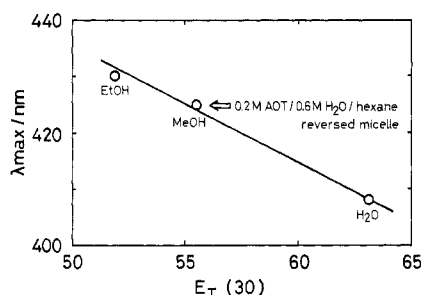
Figure 2. Absorption maxima of 2 in several polar solvents as a function of the Dimroth's solvent-polarity parameter, E_T(30) at 25.0 °C. Blank arrow shows the absorption maximum in the AOT/hexane micelle.
