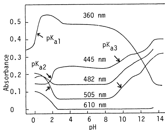
Fig. 2. pH Dependence of the absorption bands. Arrows indicate the absorbance changes used for \text{pK}_a determination.
