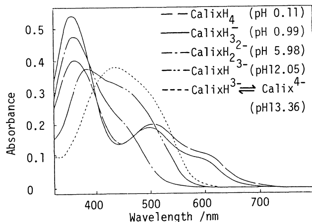
Fig. 1. Absorption spectra of \text{3(R=NMe}_3^+\text{Cl}^-) ( 1.00 \times 10^{-5} \text{ mol dm}^{-3} ) at 20^\circ\text{C} .
