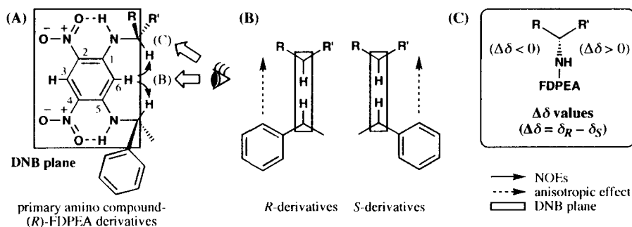
Figure 1. (A) Conformation of primary amino compound-( R )-FDPEA derivatives. (B) and (C) Views of the ( R and S )-FDPEA derivatives drawn from the direction shown by the outlined arrow in (A).
