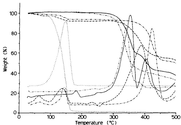
Fig. 3. TGA and DTG plots of ferrocene ( \cdots ), dppf (—), vacuum untreated (---) and treated ( -\cdots- ) \text{dppfO}_2 , and \text{dppfS}_2 (— — —).
