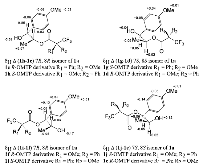
Figure 1. Chemical shift differences between diastereoisomeric pairs of compounds formed from the derivatization of threo -anethole glycol ( 1a , 7S/8S and 7R/8R ) by (S)-(+)- and (R)-(–)-MTPCl. From calculated differences ((S)-MTPA) – ((R)-MTPA) for 1g – 1d , 1j – 1e , 1h – 1c and 1i – 1f , according to the preferred conformations normally assumed for MTPA esters 8 (Figure 1), confirmed this supposition and
