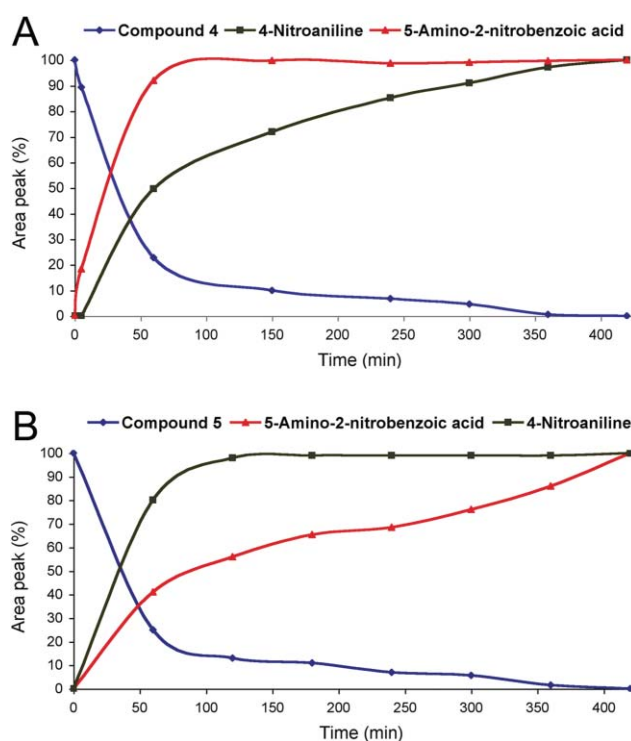
Fig. 6 PGA-catalyzed the release of 5-amino-2-nitrobenzoic acid and 4-nitroaniline from compounds 4 and 5 through 1,6- and 1,4-eliminations. Conditions: 4 or 5 , [500 \mu M] in PBS 7.4, PGA [0.01 mg mL -1 ].
