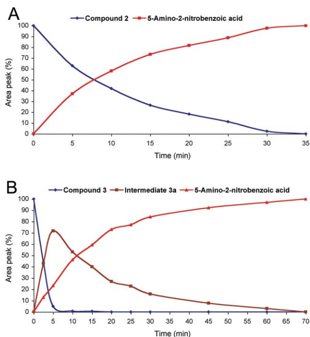
Fig. 4 PGA-catalyzed the release of 5-amino-2-nitrobenzoic acid from compounds 2 and 3 through 1,6- and 1,4-eliminations respectively. Conditions: 2 or 3 , [500 \mu M] in PBS 7.4 and PGA [0.01 mg mL -1 ].
