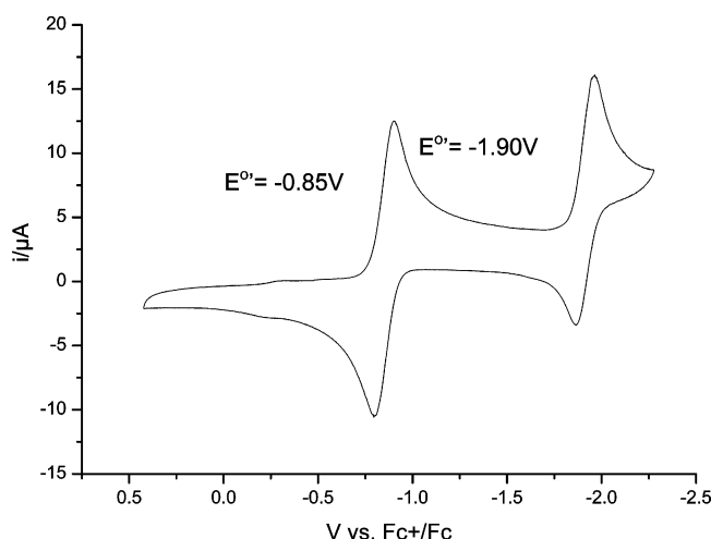
Figure 9. Cyclic voltammogram of 6 in \text{CH}_3\text{CN} , 0.1 M TBAHFP; sweep rate, 400 mV/s; -25^\circ\text{C} .
