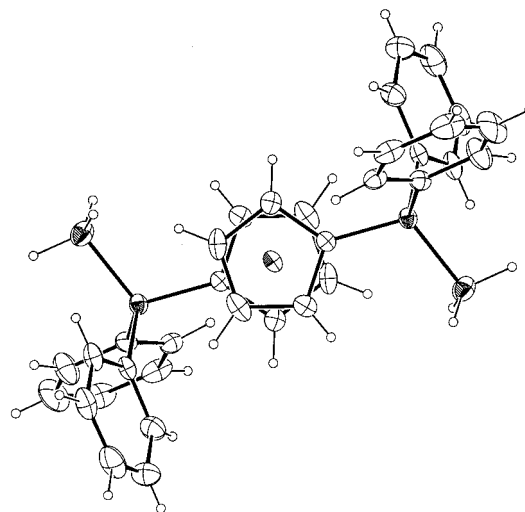
Figure 2. Alternate view of the structure of \text{dppf}(\text{BH}_3)_2 , 1 , showing the staggered anti arrangement of the cyclopentadienyl rings.
