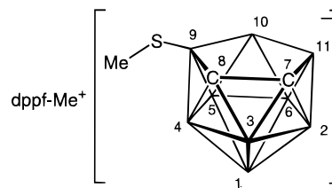
Figure 6. Proposed structure of [dppf-Me + ][ nido -9-MeS-7,8-C 2 B 9 H 11 − ], 6 .
