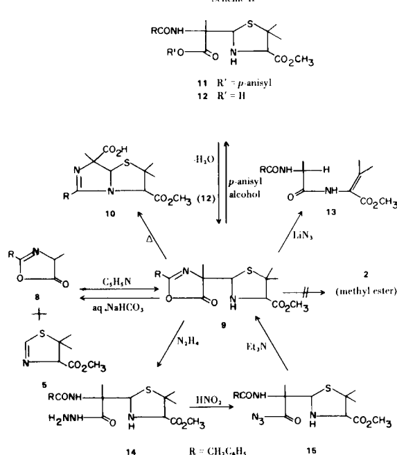
Scheme II
