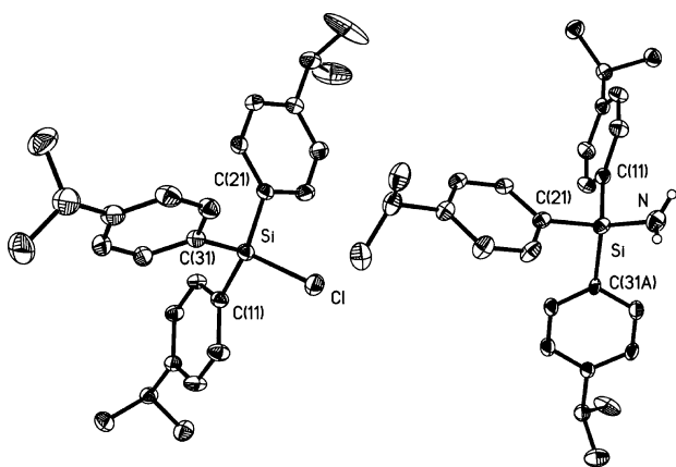
(4- i PrC 6 H 4 ) 3 SiCl 5
