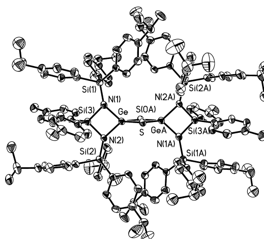
Figure 4. Molecular structure of [\{(4\text{-}^i\text{PrC}_6\text{H}_4)_3\text{SiN}]_2\text{Si}(\text{tolyl})_2\}\text{Ge}(\mu\text{-S})_2 ( 13 ) with hydrogen atoms and solvate molecules omitted for clarity. Selected bond lengths (Å) and angles (deg): Ge–S 2.2253(10), Ge–S' 2.2392(9), Ge–N(1) 1.837(3), Ge–N(2) 1.850(3), N(1)–Si(1) 1.738(3), N(1)–Si(3) 1.764(3), N(2)–Si(2) 1.741(3), N(2)–Si(3) 1.762(3); S–Ge–S' 95.14(3), Ge–S–Ge' 84.86(3), N(1)–Ge–N(2) 85.68(12), Ge–N(1)–Si(1) 142.01(18), Ge–N(2)–Si(2) 141.76(17), Ge–N(1)–Si(3) 91.85(14), Ge–N(2)–Si(3) 91.43(12), N(1)–Si(3)–N(2) 85.68(12).
