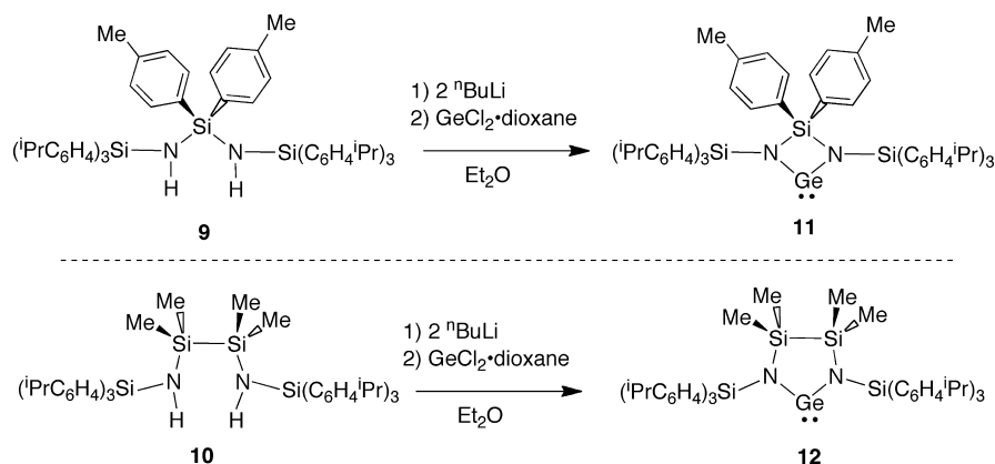
Scheme 4. Synthesis of the Germylene Complexes [\{\text{tolyl}_2\text{Si}[(4\text{-}^i\text{PrC}_6\text{H}_4)_3\text{SiN}]_2\}\text{Ge:}] ( 11 ) and [\{\text{Me}_4\text{Si}_2[(4\text{-}^i\text{PrC}_6\text{H}_4)_3\text{SiN}]_2\}\text{Ge:}] ( 12 )
