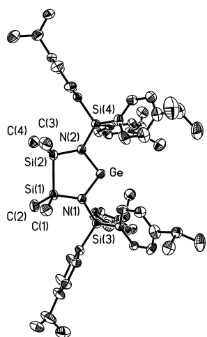
Figure 3. Molecular structure of [\{\text{Me}_4\text{Si}_2[(4\text{-}^i\text{PrC}_6\text{H}_4)_3\text{SiN}]_2\}\text{Ge:}] ( 12 ) with thermal ellipsoids at a 30% probability level. All hydrogen atoms and disordered 4\text{-}^i\text{PrC}_6\text{H}_4 groups have been omitted for clarity. Selected bond lengths [Å] and angles [deg]: Ge–N(1) 1.875(3), Ge–N(2) 1.886(3), Si(1)–Si(2) 2.3400(15), Si(1)–N(1) 1.744(3), Si(2)–N(2) 1.745(3), N(1)–Si(3) 1.732(3), N(2)–Si(4) 1.737(3); N(1)–Ge–N(2) 101.46(13), N(1)–Si(1)–Si(2) 99.30(11), N(2)–Si(2)–Si(1) 99.53(11), Ge–N(1)–Si(1) 119.99(17), Ge–N(1)–Si(3) 110.55(15), Ge–N(2)–Si(2) 119.56(17), Ge–N(2)–Si(4) 110.07(15).
