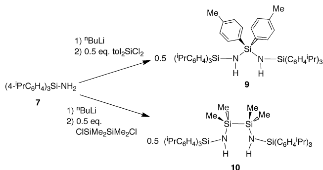
Scheme 3. Synthesis of the Silyl and Disilyl Bis(Amine) Ligand Precursors [(4- i PrC 6 H 4 ) 3 SiNH] 2 Si(tolyl) 2 ( 9 ) and [(4- i PrC 6 H 4 ) 3 SiNHSiMe 2 ] 2 ( 10 )
