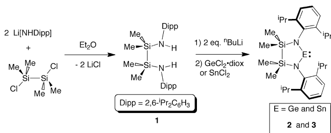
Scheme 1. Synthesis of the Bis(amido)disilyl Germylene and Stannylene Heterocycles [(\text{Me}_2\text{SiNDipp})_2\text{E}] (E = Ge and Sn; 2 and 3 )
