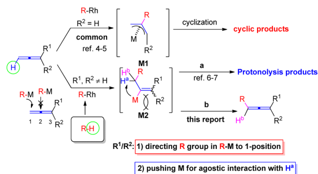
Scheme 1. Carbometallation of Allenes with R–M Species
