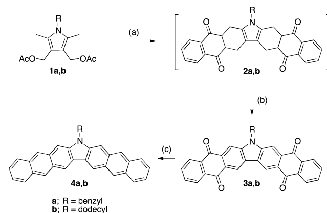
Scheme 1. Synthesis of DNCs a
