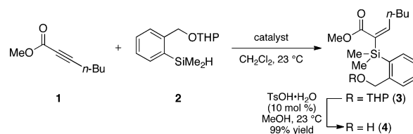
Scheme 1. Hydrosilylation/Deprotection with Silane 2
