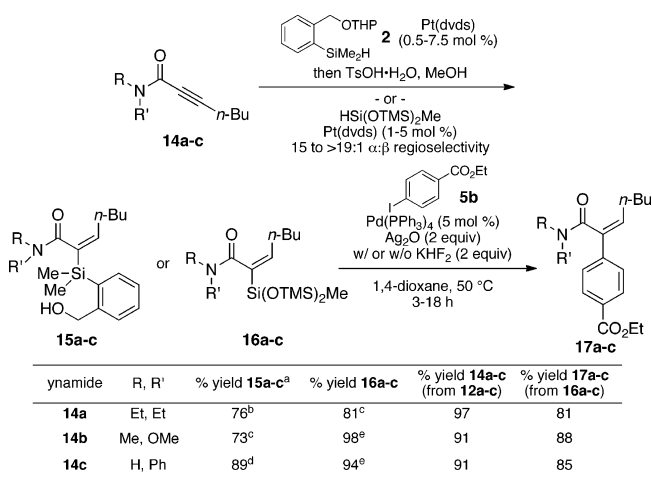
Scheme 3. Ynamide Hydrosilylation/Hiyama Couplings
