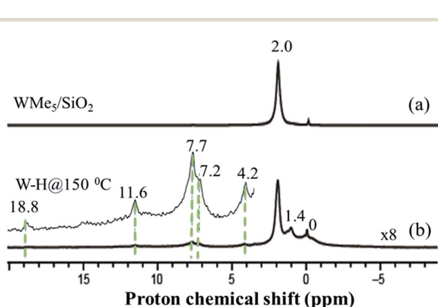
Fig. 3 One-dimensional (1D) ^1\text{H} solid-state NMR spectra recorded at room temperature for species 1 (a) and 2 (b) acquired at 500 MHz ( i.e. , within a magnetic field, B_0 , of 11.7 T) with a 10 kHz MAS frequency for (a) and 12.5 kHz MAS frequency for (b), a repetition delay of 5 s, 32 scans for (a), and 128 scans for (b).
