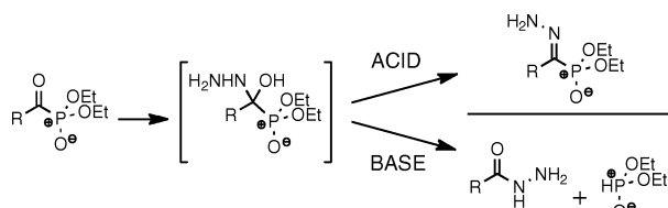
Scheme 4. Reaction Course of Acyl Phosphonates with Hydrazine is pH-Dependent
