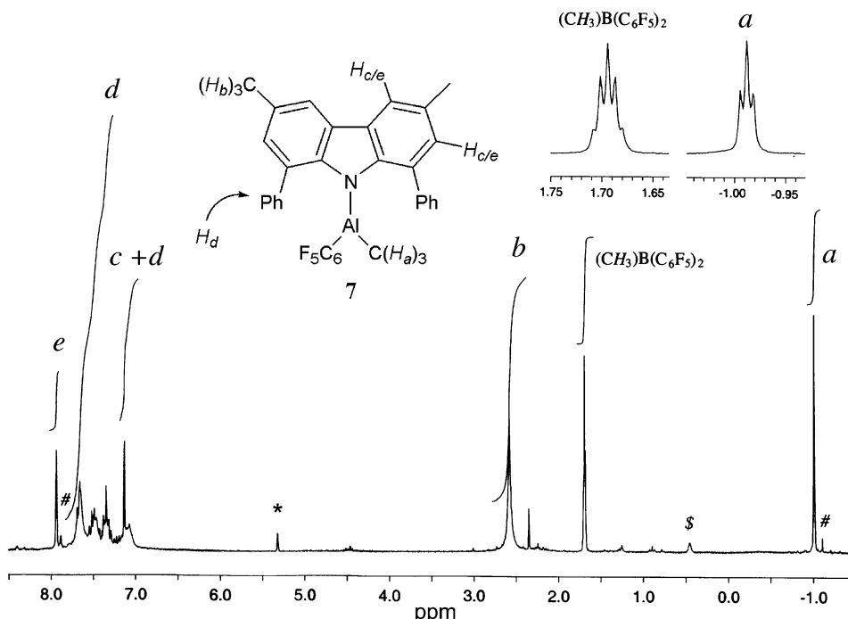
Fig. 2. ^1\text{H} -NMR spectrum ( \text{CD}_2\text{Cl}_2 ) arising from reaction of 4 with \text{B}(\text{C}_6\text{F}_5)_3 ; *, residual protio impurity in \text{CD}_2\text{Cl}_2 ; $, signal corresponding to non-coordinated anion [\text{MeB}(\text{C}_6\text{F}_5)_3]^- ; #, signals attributable to 6 .
