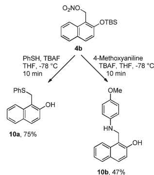
Scheme 4. Michael Addition of Thiophenol and 4-Methoxy Aniline to the in Situ Generated o -Naphthoquinone Methide
