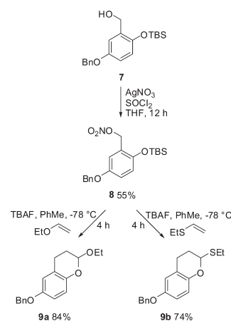
Scheme 3. Synthesis of 5-(Benzyloxy)-2-( tert -butyldimethylsilyloxy)benzyl Nitrate 8 and Its Hetero-Diels–Alder Reaction with EVE and Ethyl Vinyl Sulfide
