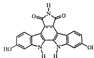
5a arcyriflavin C 5b arcyriflavin B (with double bond)
