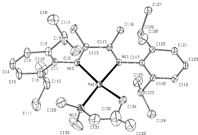
Figure 1. Molecular structure of [(\text{DAD})\text{Pd}(\text{CH}_2\text{CHMeCH}_2\text{NMe}_2)][\text{BARF}_4] ( 1 ). Thermal ellipsoids are at the 50% probability level. Selected bond distances (Å) and angles (deg): Pd11–N11 = 2.078(4), Pd11–N12 = 2.152(4), Pd11–N13 = 2.091(5), Pd11–C134 = 2.023(6), N11–Pd11–N12 = 76.67(15), N13–Pd11–C134 = 82.2(2).
