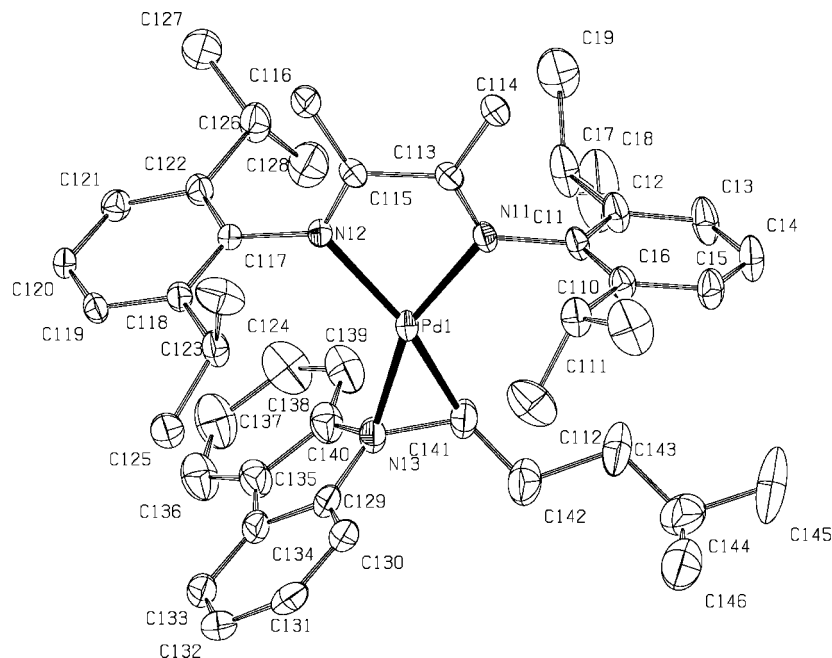
Figure 2. Molecular structure of [(\text{DAD})\text{Pd}(\eta^2\text{-Me}_2\text{CHCH}_2\text{CH}_2\text{CHNC}_{12}\text{H}_8)][\text{BARF}_4] ( 2 ). Thermal ellipsoids are at the 50% probability level. Selected bond distances (Å) and angles (deg): Pd1–N11 = 2.085(3), Pd1–N12 = 2.143(4), Pd1–N13 = 2.104(5), Pd1–C141 = 2.015(7), N13–C129 = 1.453(7), N13–C140 = 1.450(8), N13–C141 = 1.449(8), N11–Pd1–N12 = 75.32(14), N13–Pd1–C141 = 41.1(2).
