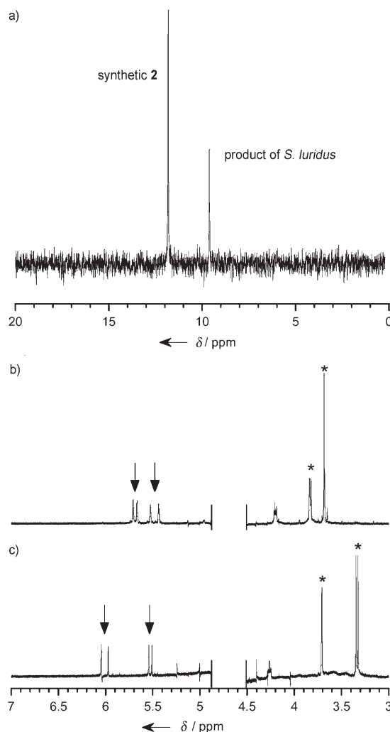
Figure 1. a) 31 P NMR spectrum of A53868 isolated from S. luridus and synthetic 2 . b) 1 H NMR spectrum of synthetic peptide 2 . c) 1 H NMR spectrum of A53868 from S. luridus . The spectra were recorded in D 2 O, and the water peak is omitted in (b) and (c) for clarity. The arrows and asterisks are explained in the text.
