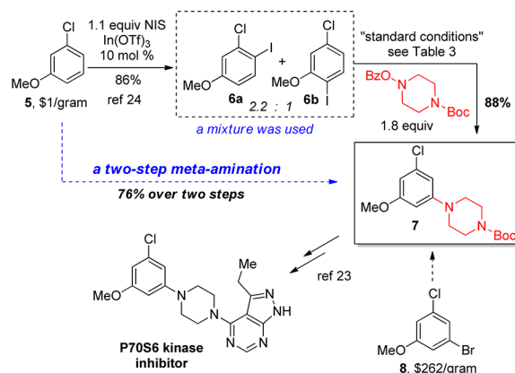
Scheme 3. Synthetic Application
