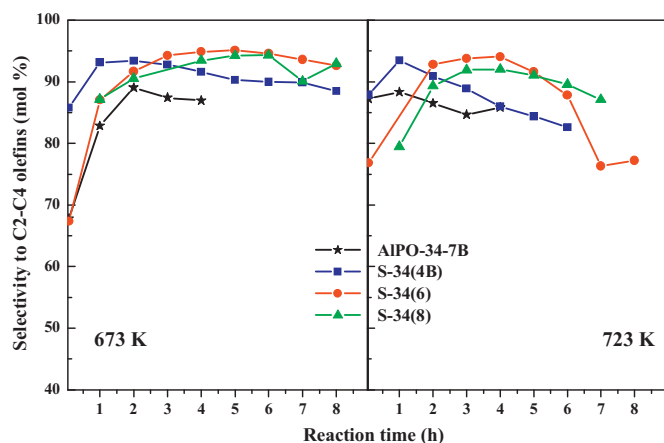
Fig. 8. Selectivity to short chain olefins (C2–C4) in function of the time on stream for the different samples in the MTO reaction. Test conditions: T=673\text{--}723\text{ K} , \text{WHSV}=1.2\text{ h}^{-1} , 1 g of catalyst.
