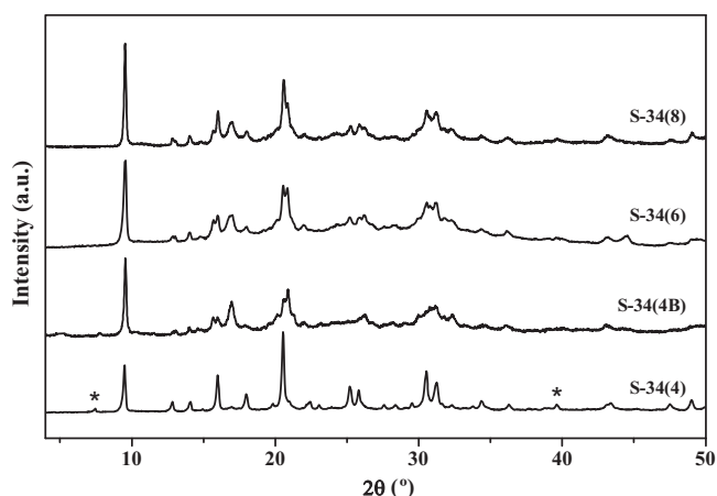
Fig. 1. X-ray diffraction patterns of SAPO-34 samples synthesized with different amount of silicon in the synthesis gel. The asterisks indicate reflections showing the presence of and additional AFI phase.
