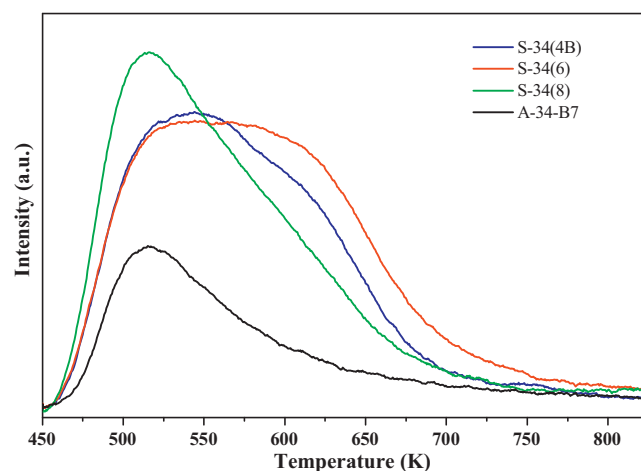
Fig. 6. \text{NH}_3 -TPD plots of calcined SAPO-34 catalysts synthesized with different amount of silicon in the synthesis gel.
