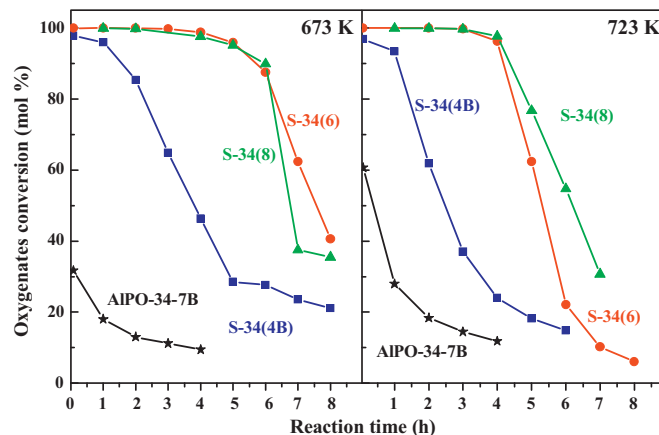
Fig. 7. Conversion of oxygenates (MeOH and DME) vs. reaction time obtained with the different catalysts. Test conditions: T = 673 – 723 K, \text{WHSV} = 1.2 \text{ h}^{-1} , 1 g of catalyst.
