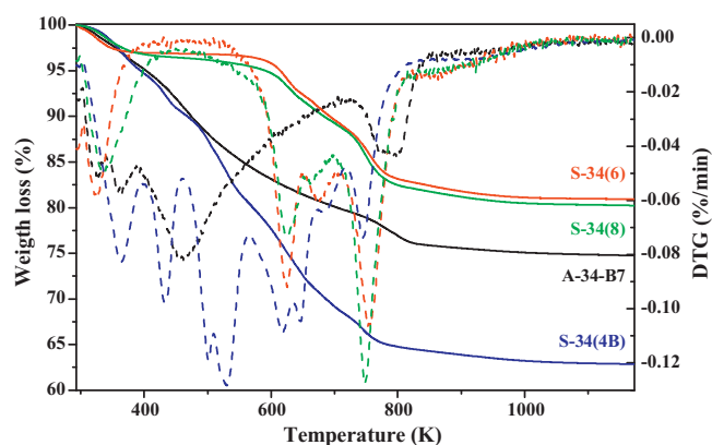
Fig. 3. Thermogravimetric analyses (solid lines) and derivatives (dotted lines) of AlPO-34 and SAPO-34 samples.
