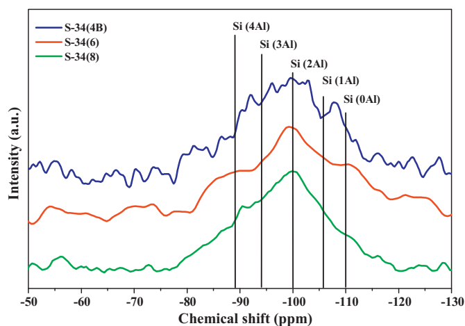
Fig. 5. ^{29}\text{Si} CP/MAS NMR spectra of calcined SAPO-34 catalysts synthesized with different amount of silicon in the synthesis gel.
