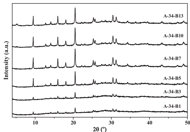
Fig. 2. X-ray diffraction patterns of AlPO-34 samples synthesized at different crystallization times.
