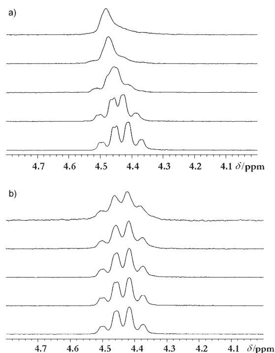
Figure 3. ^1\text{H} NMR spectra of the methylene region of host 2a in \text{CDCl}_3 as a function of a) added \text{NBu}_4^+\text{Br}^- and b) added \text{NBu}_4^+\text{CF}_3\text{SO}_3^- (bottom to top 0, 0.2, 0.5, 1.0 and 5.0 equivalents of anion).
