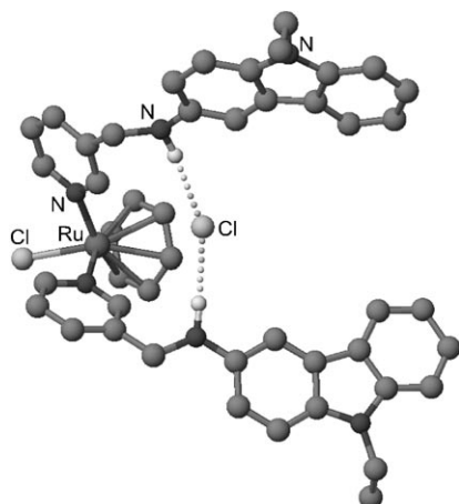
Figure 8. DFT calculated geometry for the 1:1 complex 2c-Cl - (CH hydrogen atoms omitted for clarity).
