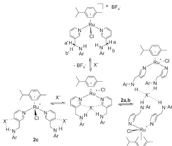
Scheme 1. Anion binding by complexes 2 forms both 1:1 and 2:1 host/guest complexes.
