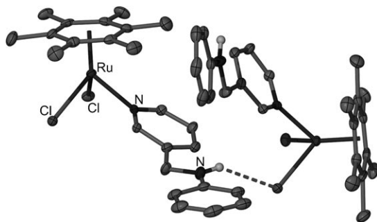
Figure 1. X-ray crystal structure of [\text{Ru}(\eta^6\text{-C}_6\text{Me}_6)\text{Cl}_2(\text{L}^1)] ( 4 ) showing the \text{NH}\cdots\text{Cl} hydrogen bonding, \text{N}\cdots\text{Cl} 3.436(3) Å (50% displacement ellipsoids).
