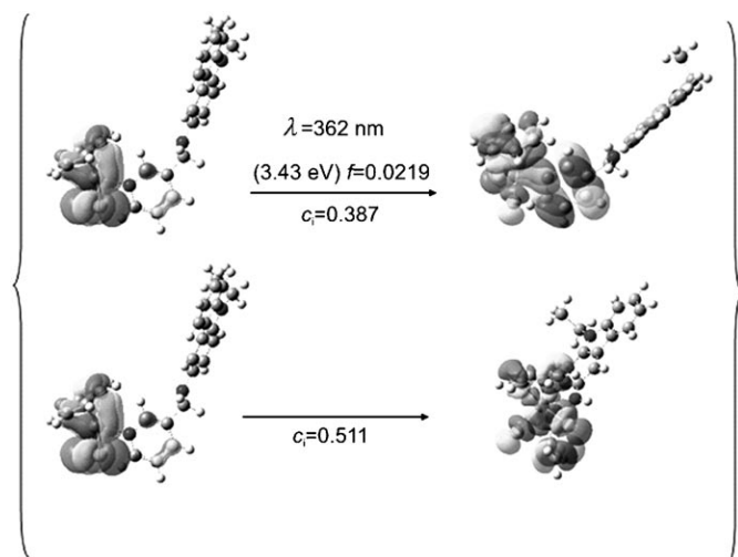
Figure 7. The first of three states giving rise to the observed \lambda = 377 nm (calcd \lambda = 362 nm) absorption in 1c . The MLCT component allows non-radiative decay and hence no fluorescence is observed.
