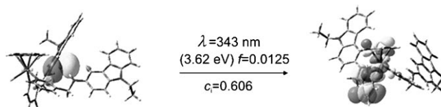
Figure 9. Charge transfer state involving \text{Cl}^- ion in 2c-Cl - .
