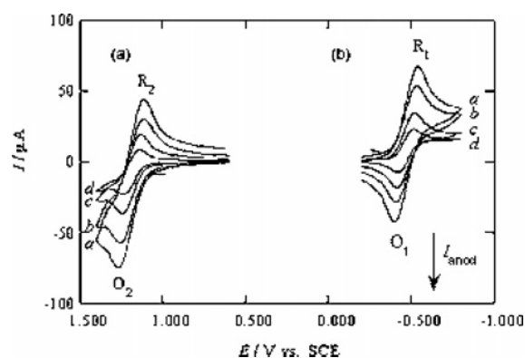
FIGURE 3. Cyclic voltammograms recorded for a 1 mM radical adduct 6 + solution in \text{CH}_2\text{Cl}_2 with TBAP 0.1 M on Pt at 25 °C. (a) Oxidation at an initial and final potential of 0.600 V and a reversal potential of 1.400 V. (b) Reduction at an initial and final potential of −0.200 V and a reversal potential of −0.800 V. Scan rate: (a) 200, (b) 100, (c) 50, (d) 20 \text{mV s}^{-1} .
