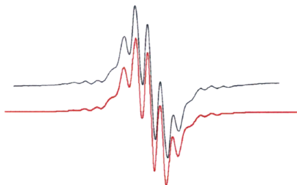
FIGURE 1. EPR spectrum of radical adduct 6* : (black) 6* in \text{CH}_2\text{Cl}_2 solution at 174 K; (red) computer simulation.
