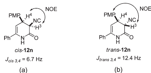
FIGURE 2. NOE correlations and H3–H4 coupling constants observed for the cis - and trans -diastereomers of 12n .
