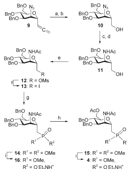
Scheme 3. Synthesis of glycosyl phosphonates 4 and 16 : a) O_3 , CH_2Cl_2 , -78^\circ C , 10 min; b) NaBH_4 , THF/H_2O 7:3, -78^\circ C \rightarrow RT , 95% over two steps; c) PPh_3 , THF , RT , 3 h, then H_2O , 14 h; d) Ac_2O , MeOH , RT , 30 min, 96% over two steps; e) CH_3SO_2Cl , Py , CH_2Cl_2 , RT , 24 h, 88%; f) NaI , butanone, 100^\circ C , 16 h; g) P(OMe)_3 , 100^\circ C , vacuum, 42 h, 84% from 12 ; h) ZnCl_2 , Ac_2O/AcOH 2:1, RT , 16 h, 92%; i) Et_3N , PhSH , THF , RT , 24 h: 4 (89%), 16 (93%).
