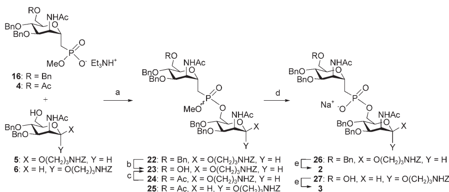
Scheme 5. Synthesis of phosphonoester-bridged dimers of MenA CPS. a) PPh 3 , DIAD, THF, 0°C → RT, 24 h: 22 (97%), 24 (90%), 25 (84%); b) ZnCl 2 , Ac 2 O/AcOH 2:1, RT, 36 h, then NaOMe, MeOH, RT, 18 h, 70%; c) NaOMe, MeOH, RT, 14 h, 76%; d) dimer 26 (from 22 ): Et 3 N, PhSH, toluene, reflux, 36 h, then MeOH, Amberlite IR-120 resin (Na + form), 95%; dimer 27 (from 25 ): NaOMe, MeOH, RT, 6 h, then DBU, PhSH, THF, RT, 7 h, then MeOH, Amberlite IR-120 resin (Na + form), 75%; e) MeOH/H 2 O 1:1, 10% Pd/C, H 2 , then H 2 O, Dowex 50W X8 resin (H + form), then Dowex 50W X8 resin (Na + form): 2 (96%), 3 (92%). DBU = 1,8-diazabicyclo[5.4.0]undec-7-ene, DIAD = diisopropyl azodicarboxylate.
