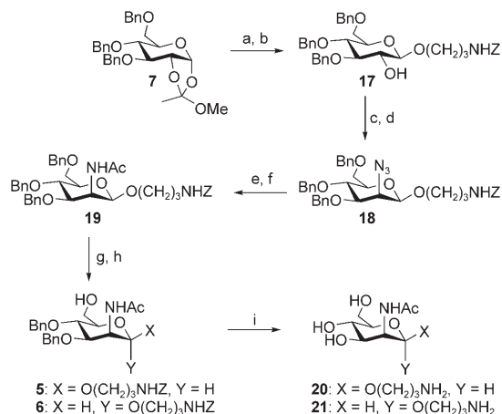
Scheme 4. Synthesis of spacer-bearing mannopyranosides. a) Benzyl N -(3-hydroxypropyl)carbamate, TMSOTf (cat.), CH 2 Cl 2 , 0°C, 2.5 h; b) NaOMe, MeOH, RT, 2 h, 85% over two steps; c) Tf 2 O, Py, CH 2 Cl 2 , 0°C, 30 min; d) Bu 4 N + N 3 - , toluene, 55–60°C, 24 h, 64% over two steps; e) PPh 3 , THF, RT, 3 h, then H 2 O, 14 h; f) Ac 2 O, MeOH, RT, 30 min, 93% over two steps; g) ZnCl 2 , Ac 2 O/AcOH 2:1, RT, 2–4 h for 5 , 24 h for 6 ; h) NaOMe, MeOH, RT, 1 h; 5 (74% over two steps), 6 (50% over two steps); i) MeOH/H 2 O 1:1, 10% Pd/C, H 2 : 20 (95%), 21 (96%).
