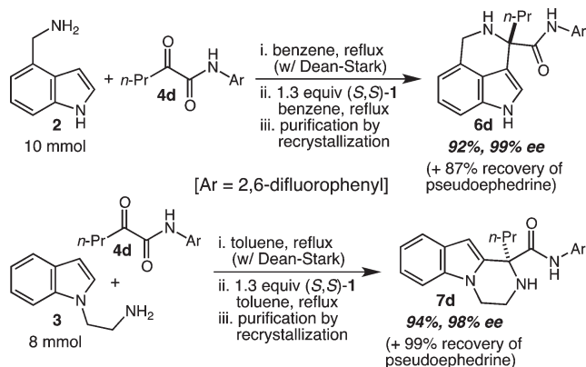
Scheme 3. “Large” Scale (8–10 mmol) Reactions with Product Isolation by Recrystallization and Pseudoephedrine Recovery by Extraction Demonstrate the Utility and Practicality of the Iso-Pictet–Spengler Reactions
