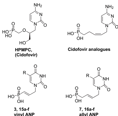
Figure 1. Some bioactive acyclic nucleoside phosphonates and our target compounds.
