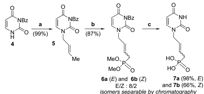
Scheme 2. Reagent and conditions: (a) crotyl bromide, K 2 CO 3 , DMF; (b) dimethyl allyl phosphonate (4 equiv), [Ru]=catalyst (5 mol %), CH 2 Cl 2 , reflux; (c) TMSBr (4.0 equiv), CH 2 Cl 2 .
