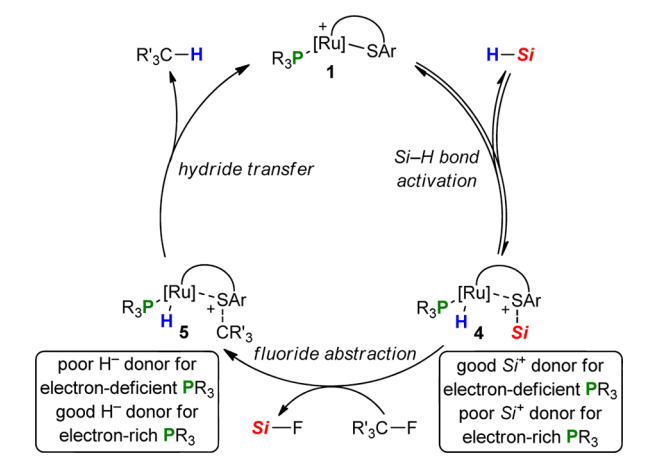
Scheme 2. Elementary Steps of the Ru–S-Catalyzed Hydrodefluorination with Silanes (BAR F 4 − as Counteranion Omitted for Clarity)
